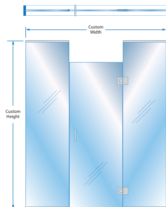
Full Height / Channel System
