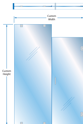
Wall Hinge / Clip System
