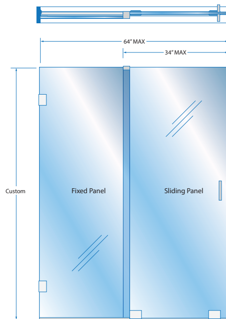
Sliding door and fixed panel with square system
