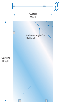
Spray panel with clip system
