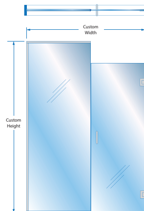
Wall Hinge / Channel System
