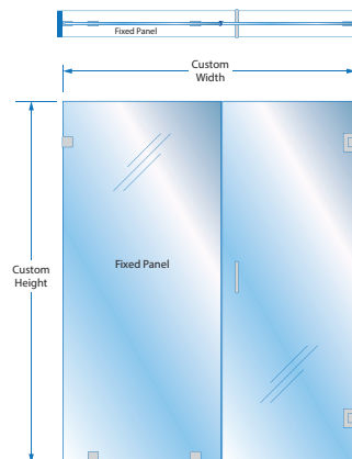
Wall Hinge / Clip System
