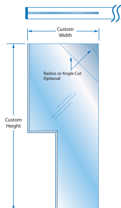
Notched spray panel with channel system
