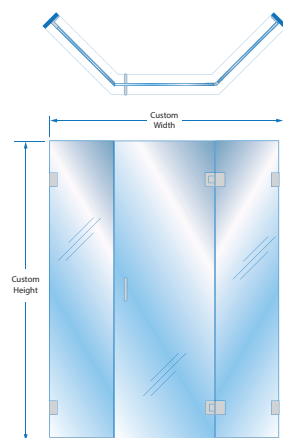
Glass-to-Glass Hinges / Channel / Clips
