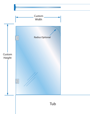
Spray panel with hinge system
