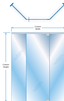
Pivot Hinge / Header/Channel
