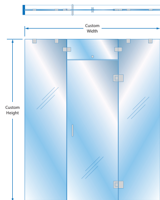
Transom / Clip & Channel System
