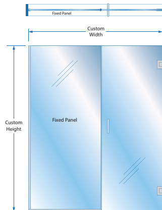
Wall Hinge / Channel System
