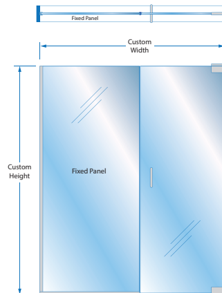
Pivot Hinge / Channel System
