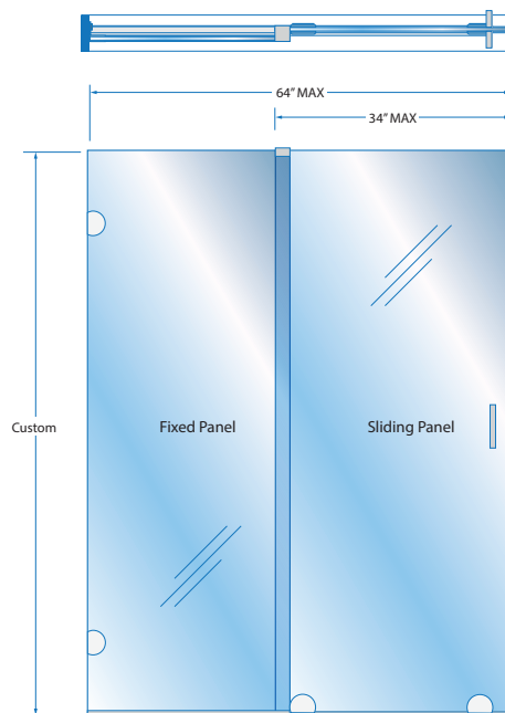
Sliding door and fixed panel with round system
