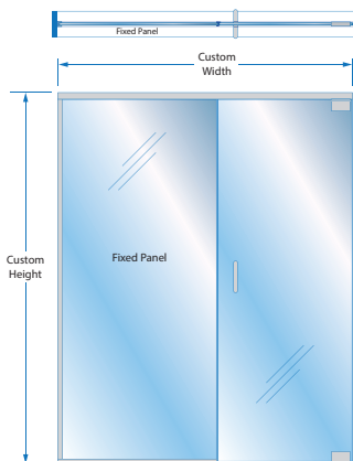
Pivot Hinge / Channel & Header
