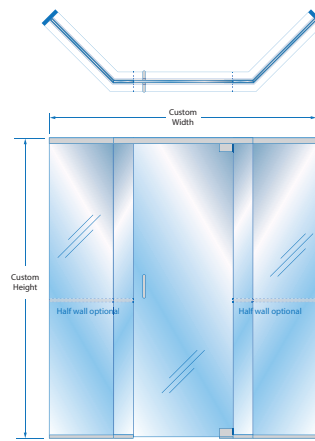
Custom / Header & Channel System
